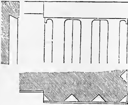
FIG. 63.—DETAILS OF THE TRIGLYPH.
